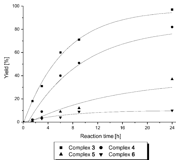
Figure 9. Yield of diphenylmethanol against time for the hydrogenation of benzophenone. Conditions: 2 mmol of benzophenone, 0.004 mmol precatalyst, 10 mL of i PrOH, reflux (82 °C), 0.008 M in KOH, substrate/KOH/complex ratio of 500:20:1.
