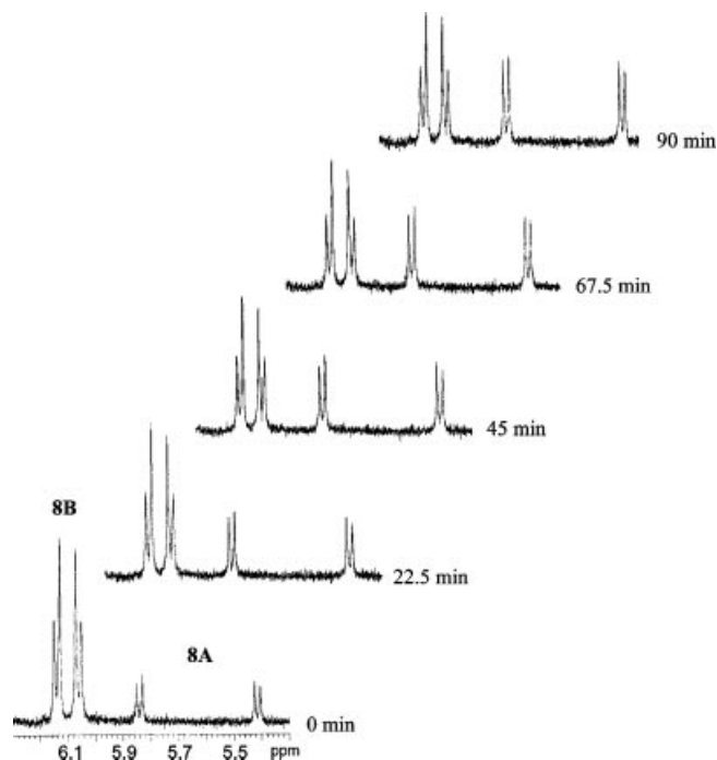
Figure 1. ^1H NMR monitoring of the evolution of a 8A / 8B mixture with time.
