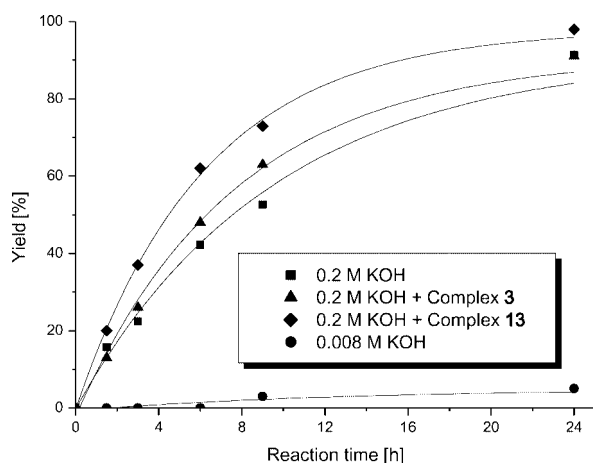
Figure 8. Yield of diphenylmethanol against time for the hydrogenation of benzophenone. Conditions: 2 mmol of benzophenone, 10 mL of i -PrOH, reflux (82 °C), 0.004 mmol precatalyst (when applicable).
